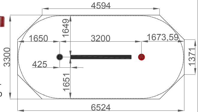
SAFER SURFACE (1/2 UNIT) (all dimensions in mm)
